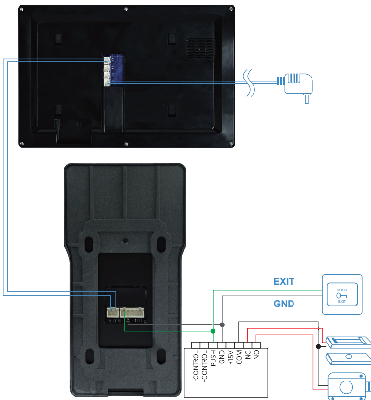
Access Control Power Connection Diagram
