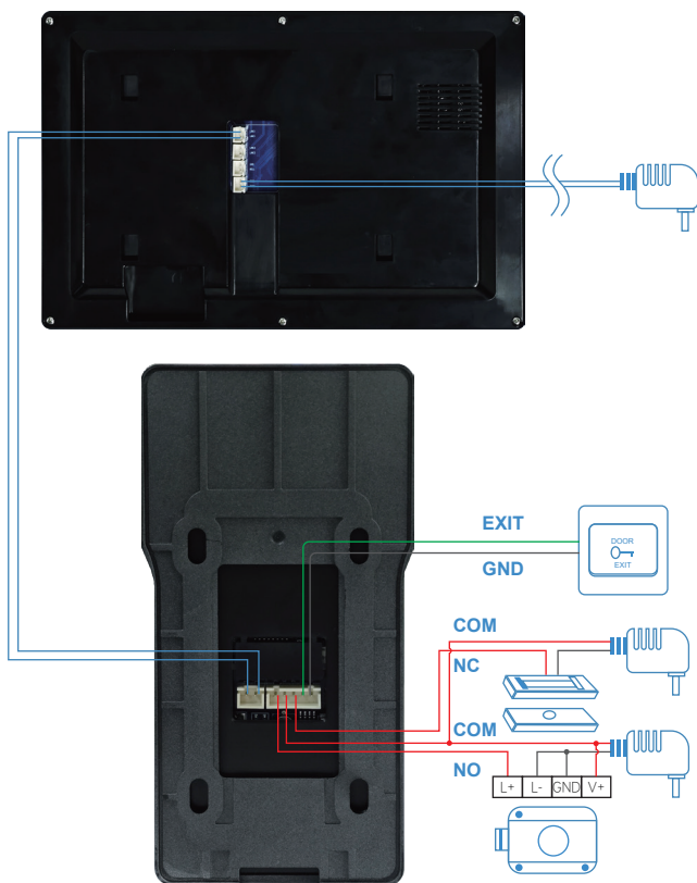
Standard Connection Diagram
