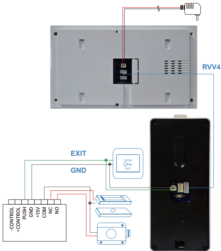
Access Control Power Connection Diagram
