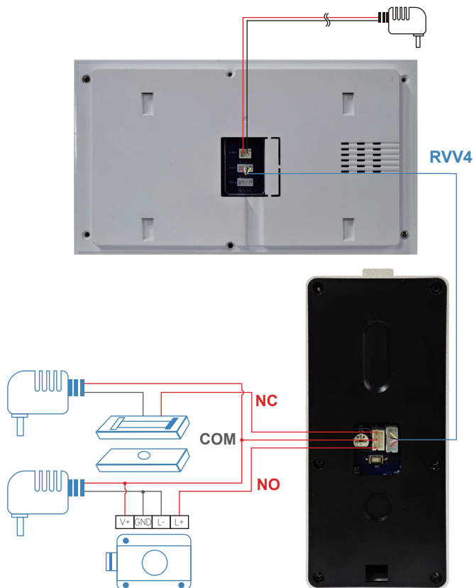
Standard Connection Diagram
